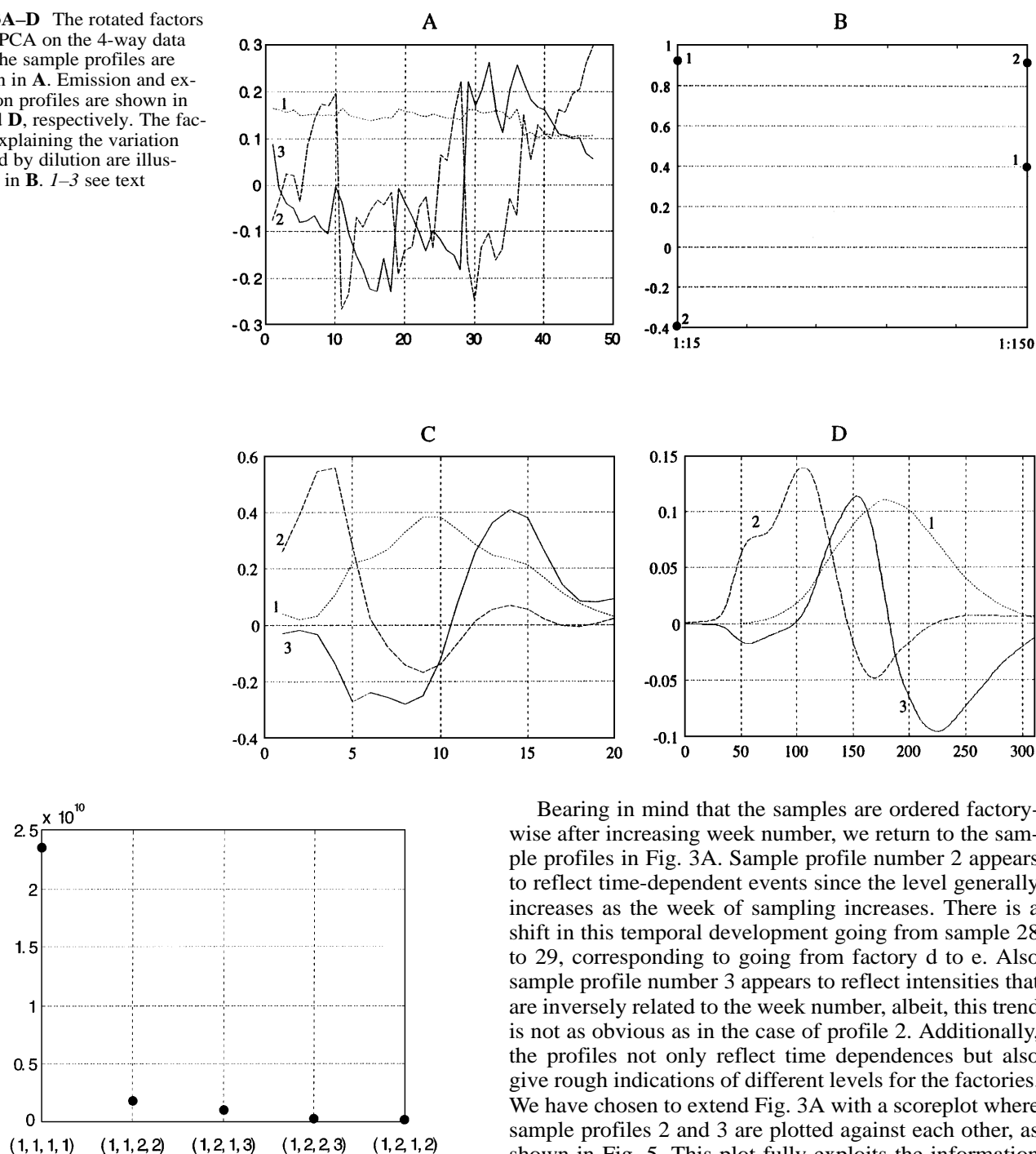
Fig. 4 The 5 largest squared elements of the core array. The remaining 49 elements are in the same range, or lower, than the lowest two elements shown here. Hence, the three most significant factor combinations are (1,1,1,1), (1,1,2,2) and (1,2,1,3)
