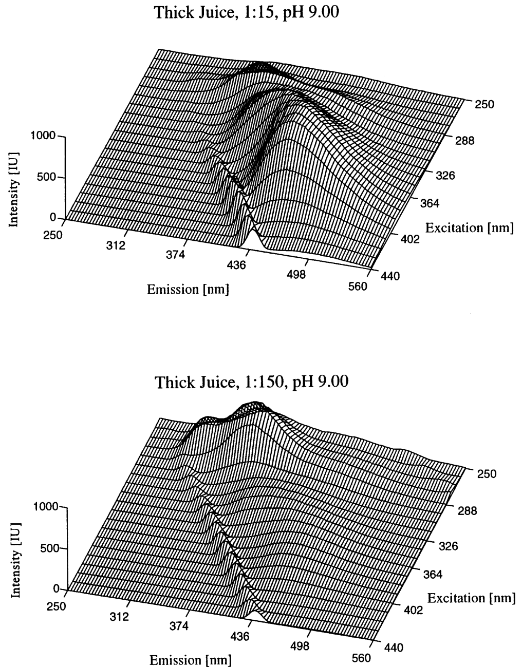
Fig. 1 Two fluorescence landscapes – one for each dilution – are measured per thick juice sample
